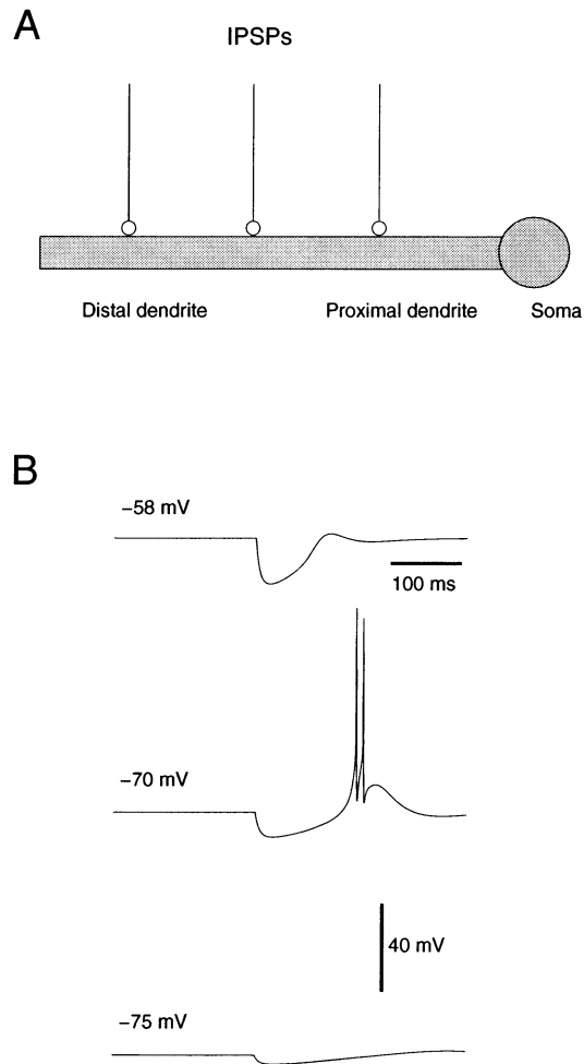
Figure 6. Voltage-dependence of IPSP-rebound sequences in a model thalamic relay cell. A. Scheme indicating that IPSPs were distributed uniformly in the dendrites of the modelled TC cell (same geometry as in figure 2A). B. IPSP obtained in the soma from activating dendritic GABA A receptors (total conductance of 10 nS). The tree traces show the effect of the same GABAergic conductance at three different resting membrane potentials. For a fixed IPSP amplitude, rebound bursting activity was only obtained within a definite range of membrane potential, because of the activation kinetics of the low-threshold calcium current I_T . The kinetics and dendritic location of I_T were modelled as in [28].
