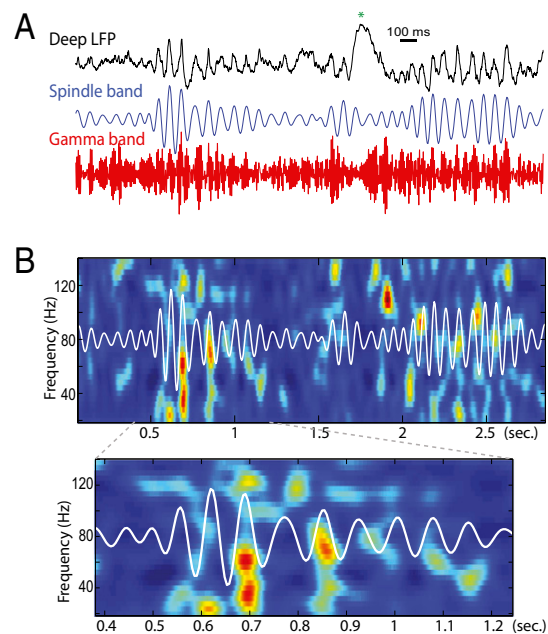
Fig. 4. Example of phase-relationship between spindle oscillations and \gamma -burst in the mPFC. (A) Raw LFP trace (Top, black) filtered in the spindle band (Middle, blue), and 30- to 140-Hz \gamma -band (Bottom, red). The green asterisk indicates a \delta -wave. (B) Time-frequency analysis in the \gamma -band reveals the occurrence of \gamma -bursts at different frequencies that tend to appear at the peak of the deep-layer spindle oscillations, as shown in the enlarged panel.
