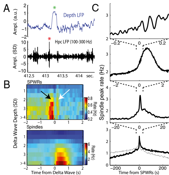
Fig. 2. Interrelationship between SPWRs, spindles, and the neocortical slow oscillation at various timescales. (A) Example of simultaneous unfiltered mPFC LFP (Upper trace, green asterisk indicates a \delta -wave) and hippocampal LFP in the pyramidal layer filtered in the ripple band (Lower trace, red asterisk indicates a detected SPWR; signal is z-scored). (B) Cross-correlograms of \delta -waves (reference) and SPWRs occurrence time in function of depth of the \delta -wave (expressed in z-score of the filtered LFP in the 0.1–4 Hz band) ( SI Materials and Methods ). All \delta -waves above 4 SD are grouped in the last row. Colors indicate occurrence rate. (C) Same as A but for spindle peaks. (C) Cross-correlograms between SPWRs (reference) and spindle peaks at various timescales, from fine (Top) to long timescales (Bottom). The thin gray line in the bottom panel is the time-reversed correlogram displayed to emphasize the difference between negative (Left) and positive (Right) time-lag differences. Only long SW5 episodes (>12 min) were used for the last cross-correlation.
